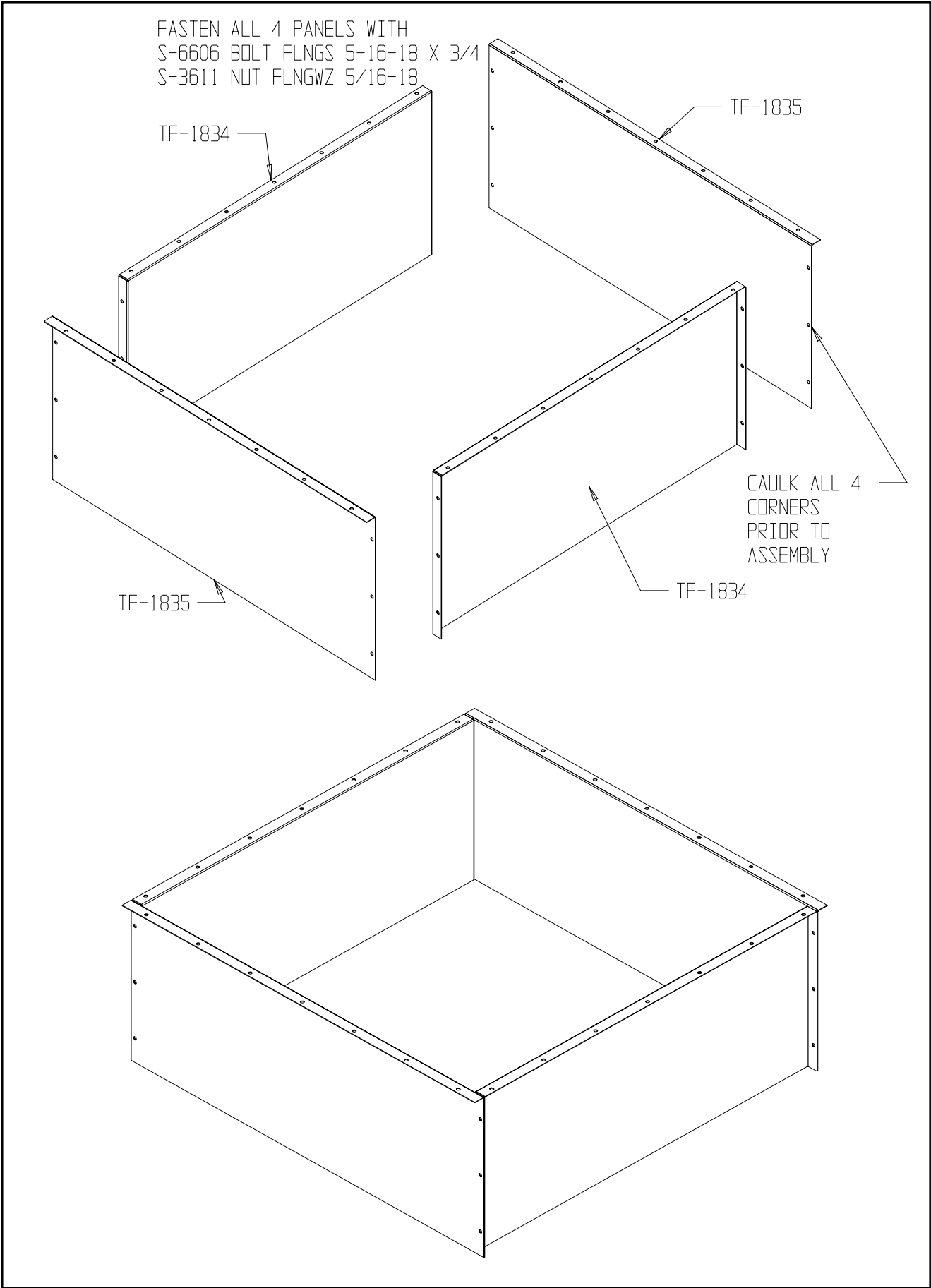
32" Duct Section
