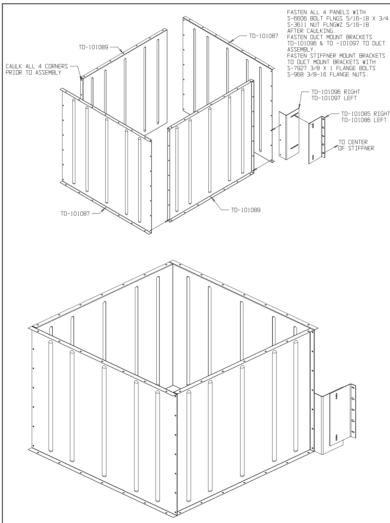
44" Duct Section
