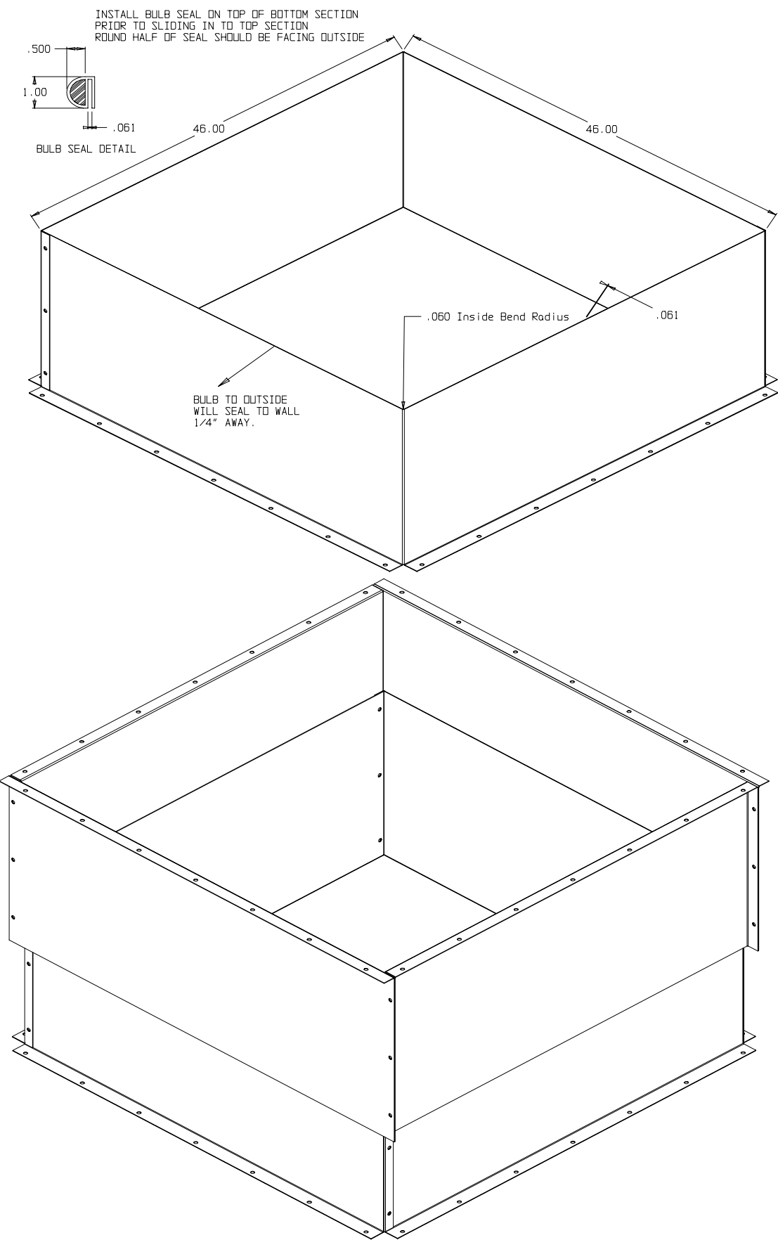
32" Duct Section
