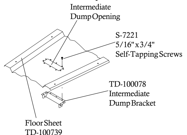
S-7221 5/16" x 3/4" Self-Tapping Screws
