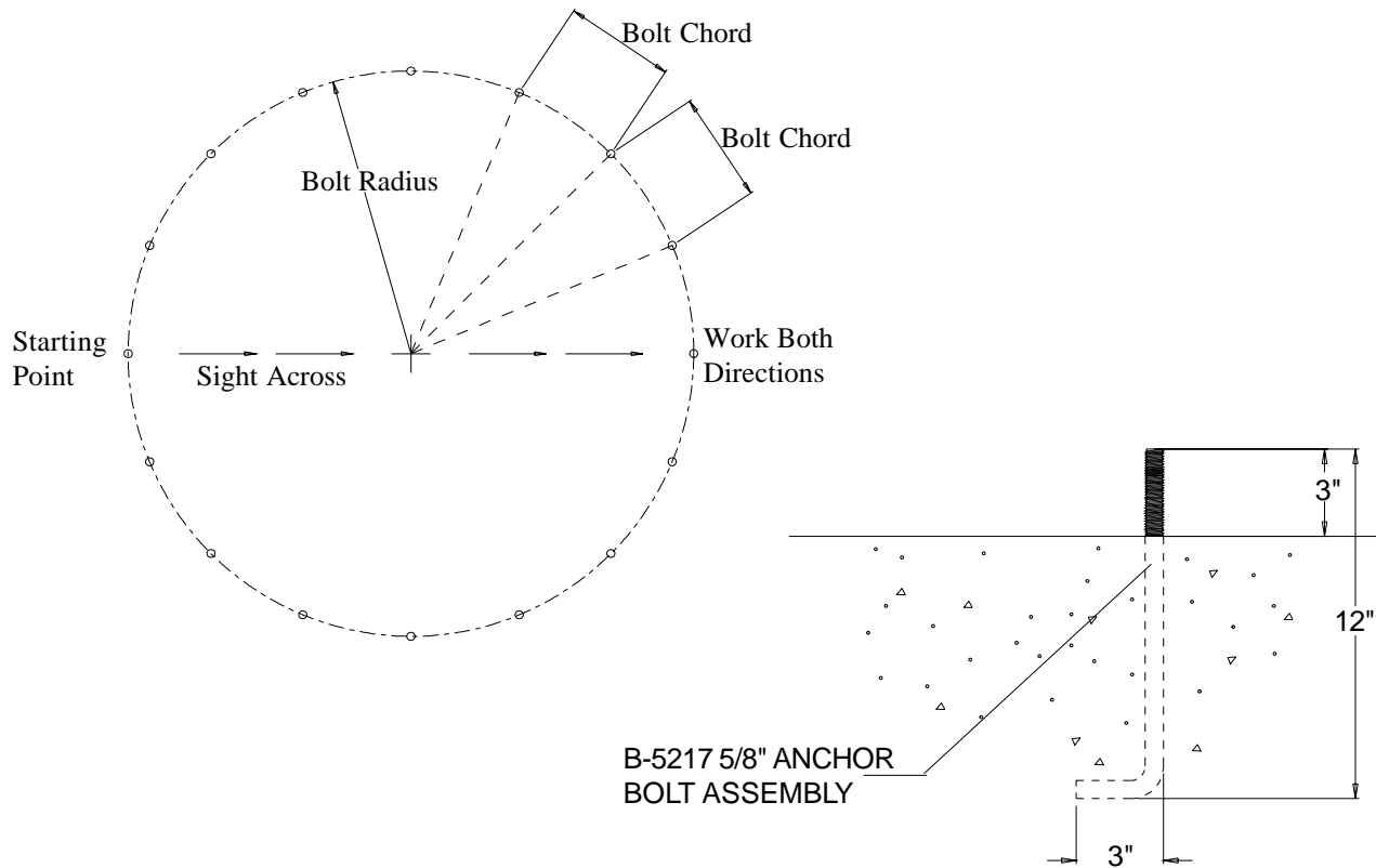
Figure #6 5/8" Anchor Bolt Detail
