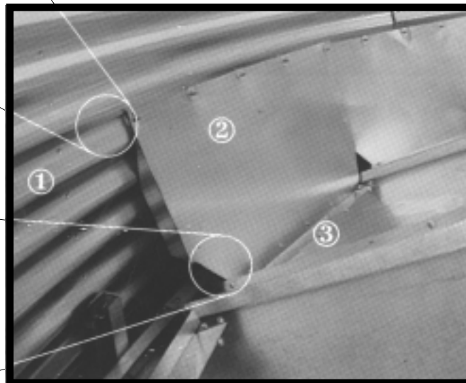
Figure #30. Flashing Attachment. 1) Sidewall, 2) Flashing TD-100648, 3) Floor sheet, 4) 5/16" x 1.1/4" bin bolt. Note that there is a nut in between the sidewall sheet and the flashing sheet.
