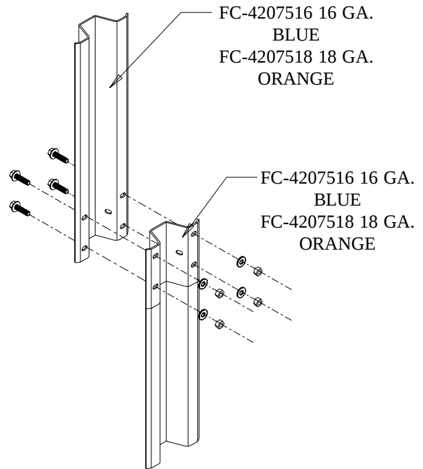
OFFSET JOINT CONNECTION DETAIL
