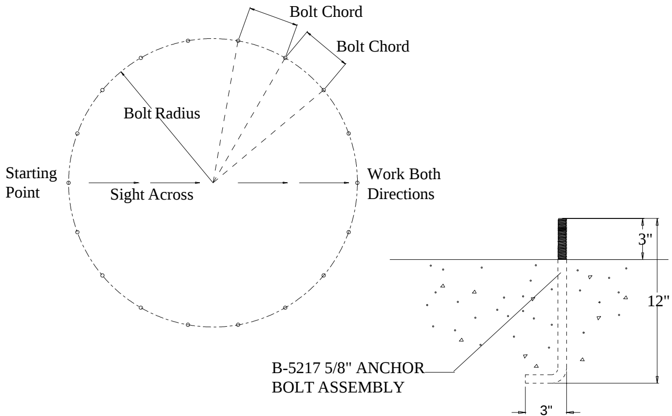
Figure #5 5/8" Anchor Bolt Detail
