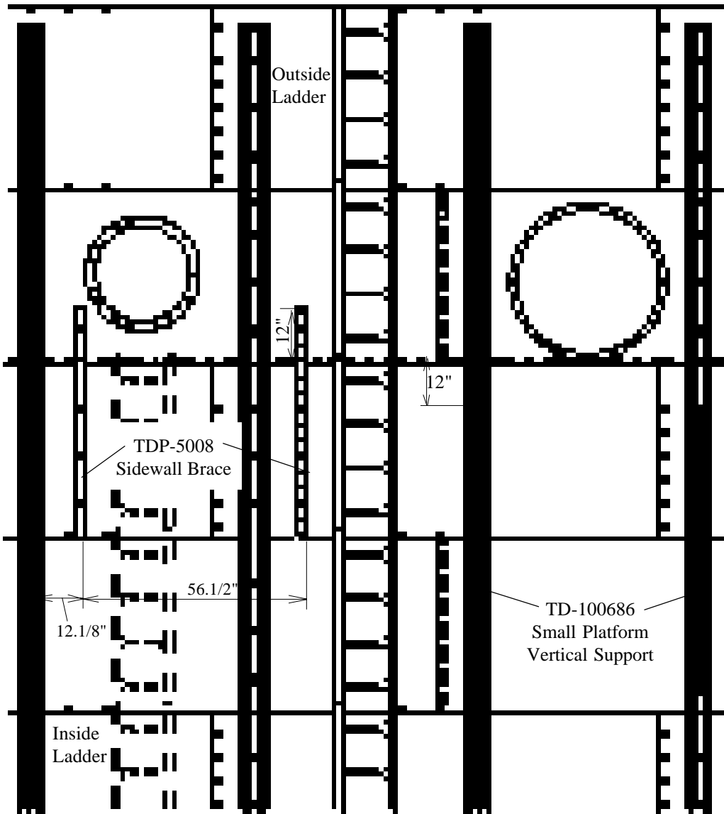
Access Door Platform
