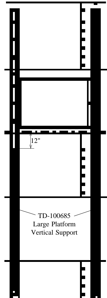
Large Platform (Optional)
