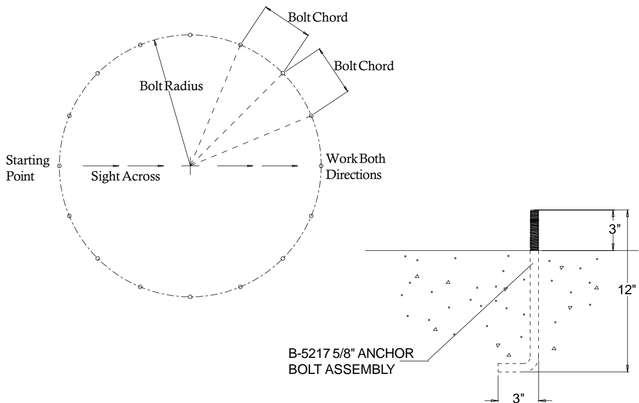
Figure #5 5/8" Anchor Bolt Detail
