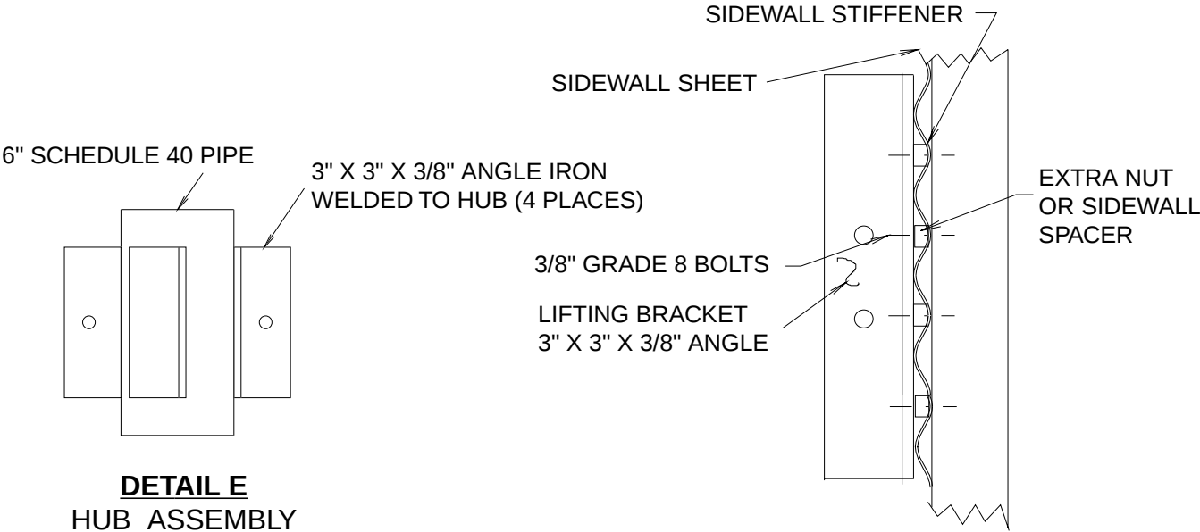
DETAIL F
