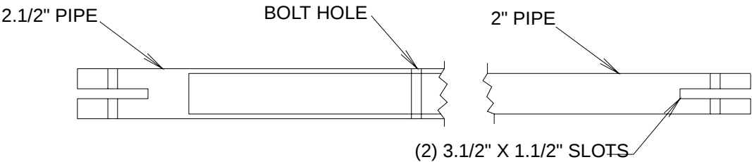
DETAIL D
