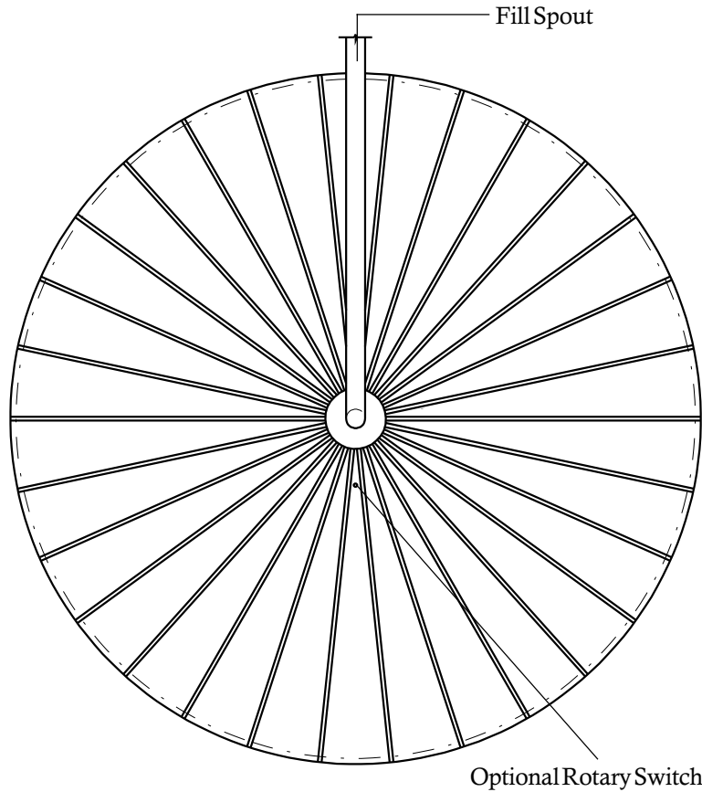
Overhead View of optional rotary Switch Locations
