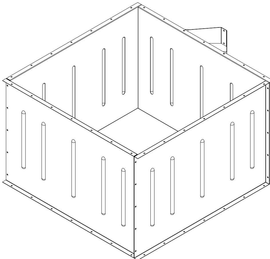
32" Duct Section
