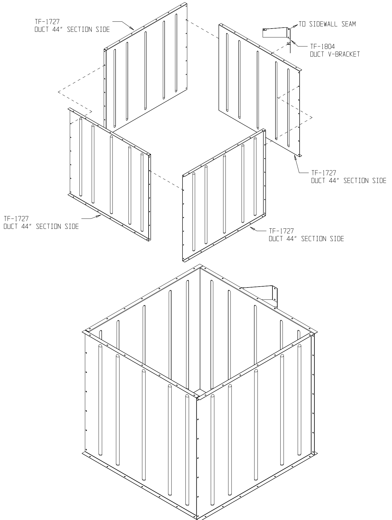
44" Duct Section
