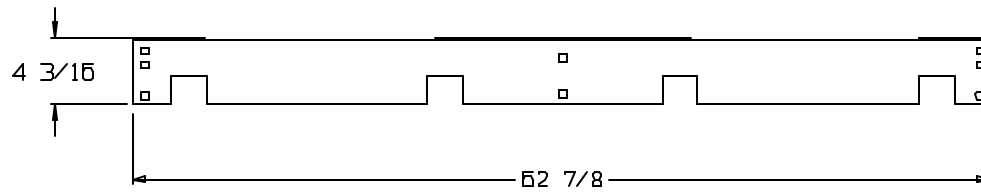
RSP36008 TOP & MID HANDRAIL (FRONT & REAR) 30' & 36' REST PLATFORM
