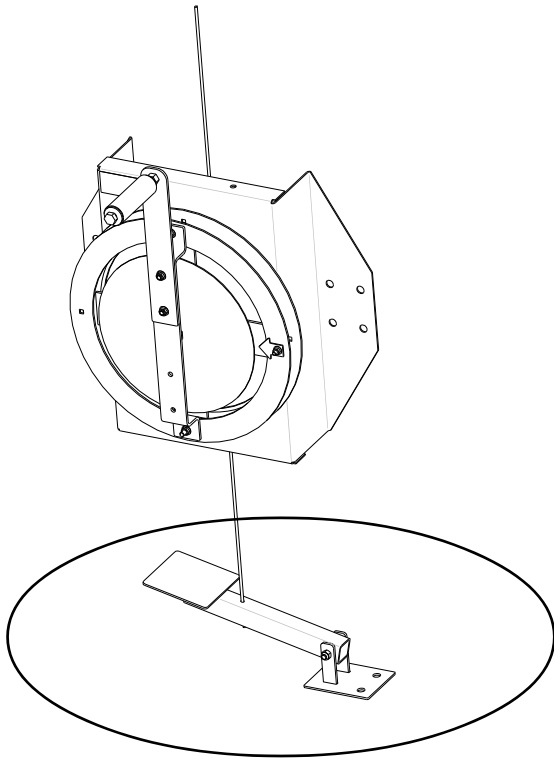
(2) Cable Clamps
