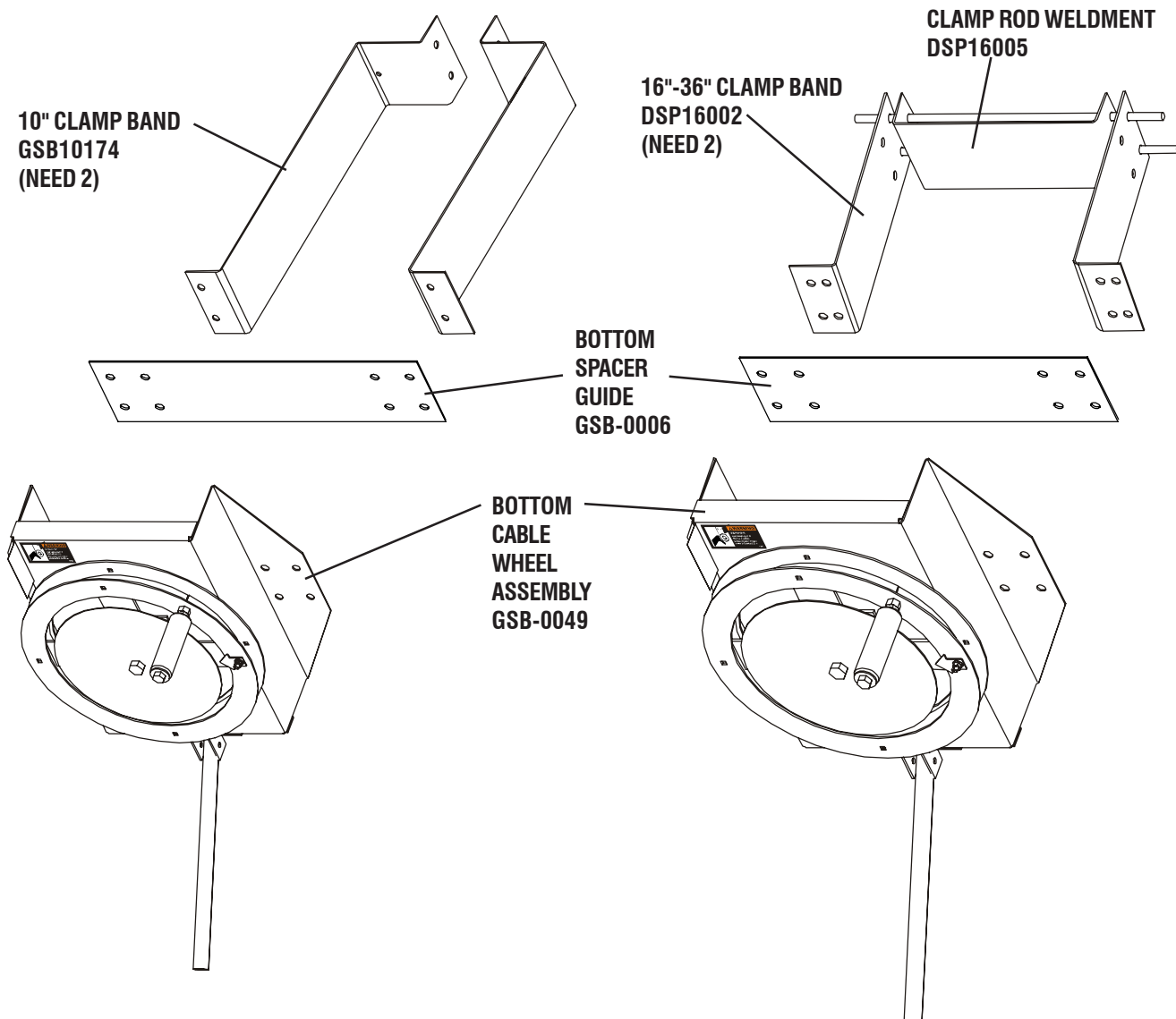
Figure 8 Trunking removed for clarity.
