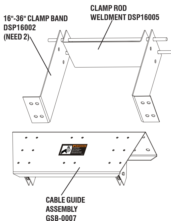
Figure 5 Trunking removed for clarity.
