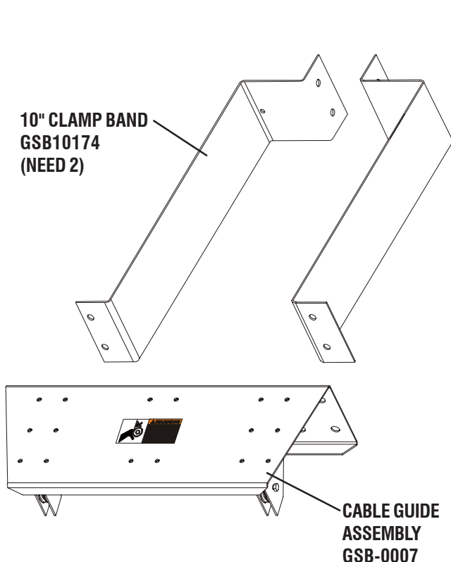
Figure 4 Trunking removed for clarity.
