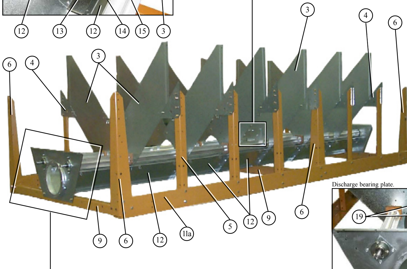
Dryer frame and lower basket assembly (view from the rear end of the dryer looking up the right side).
