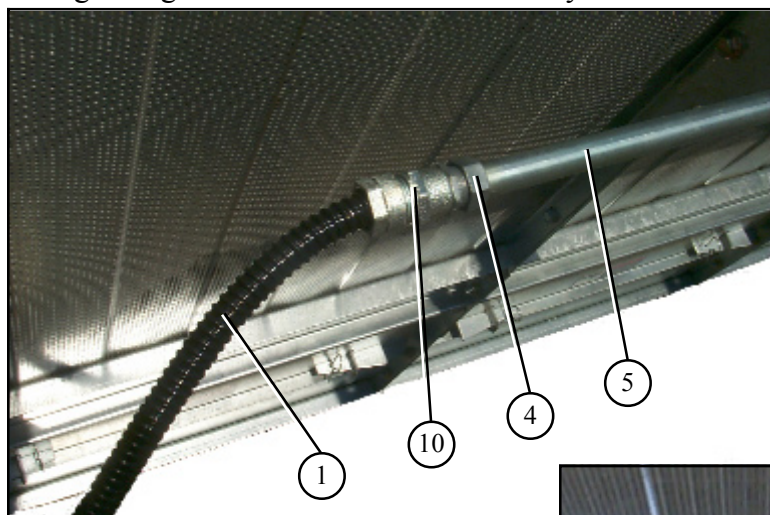
Meter roll speed sensor and rear discharge switch conduit. This is a photo of the front section of the conduit that runs through the gussets on the left side of the dryer.
