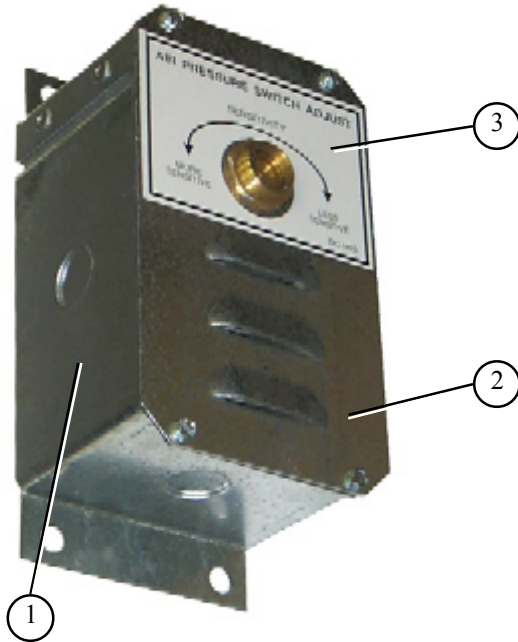
Upper air switch assembly (installed).
