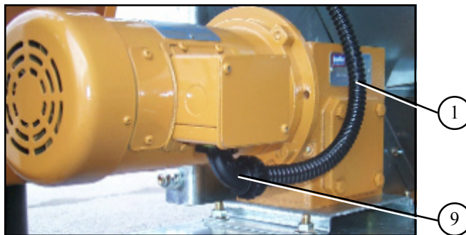
Meter roll speed sensor and rear discharge switch conduit. This is a photo of the front section of the conduit that runs through the gussets on the left side of the dryer.
