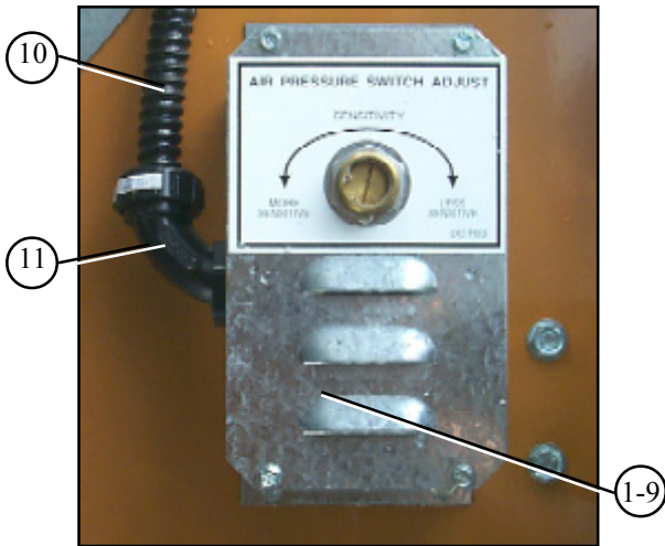
Upper air switch assembly (installed).
