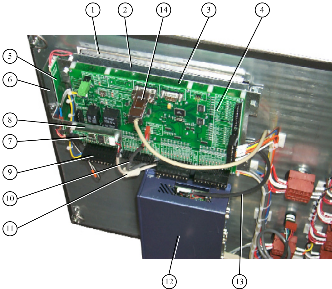
CONTROL BOX SWITCH PANEL (REAR)
