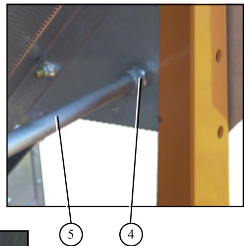
Rear discharge switch conduit at rear left gusset where 1/2" EMT conduit terminates.
