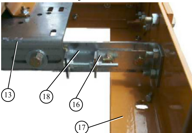
Rear drive tension adjustment.
