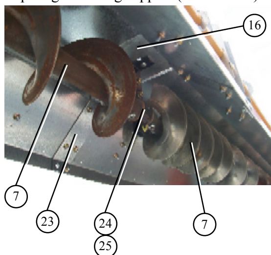
Top Auger bearing support (inside view).
