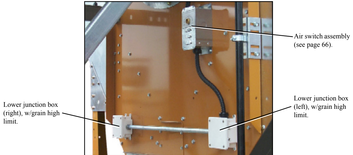
Lower junction box (right), w/grain high limit.
