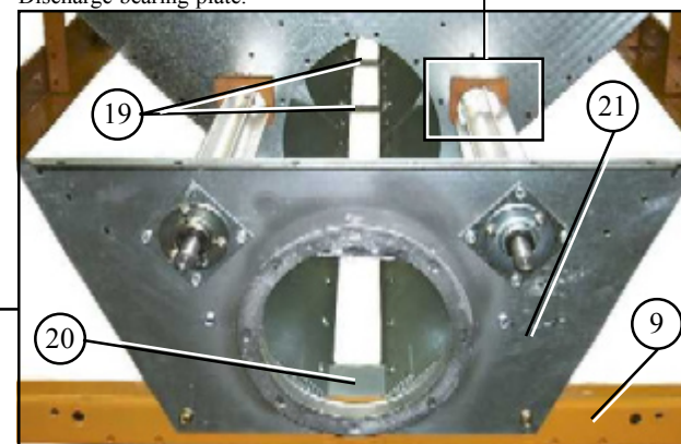
Discharge bearing plate.
