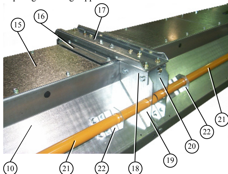
Top Auger bearing support.
