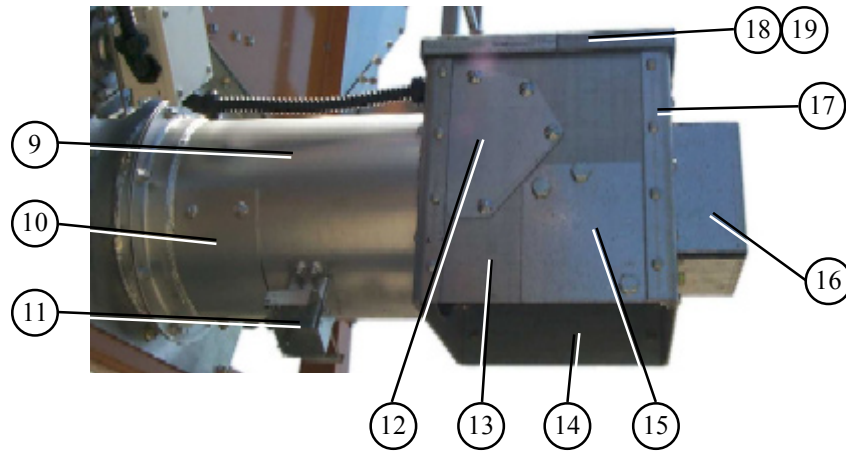
Rear Discharge Box.
