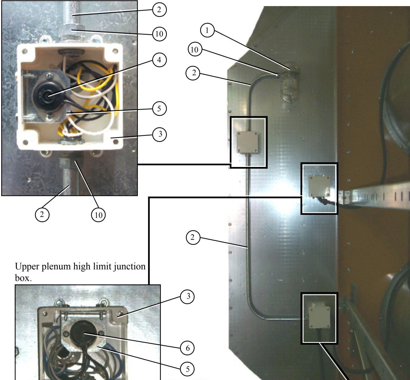
Lower plenum high limit junction box.
