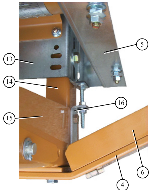
Forward drive tension adjustment.
