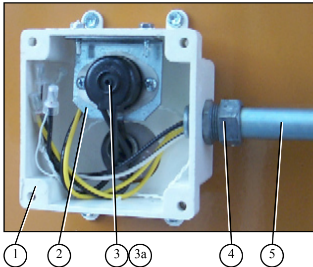
Lower junction box (right), w/grain high limit.
