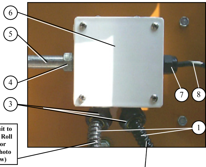
Lower junction box (left).
