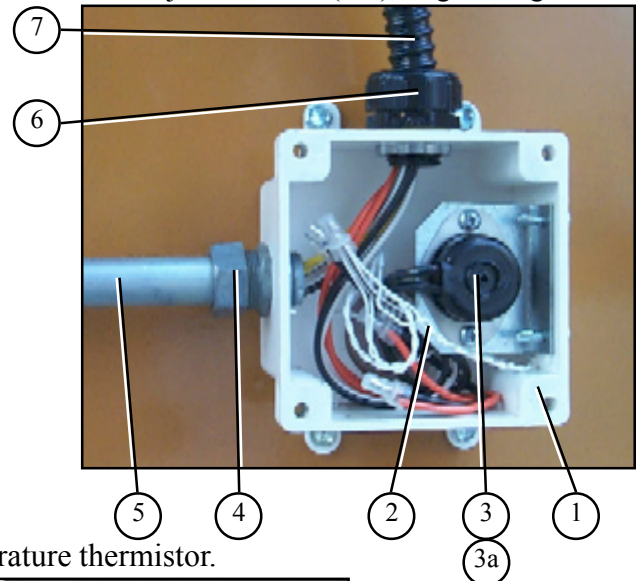
Lower junction box (left), w/grain high limit.
