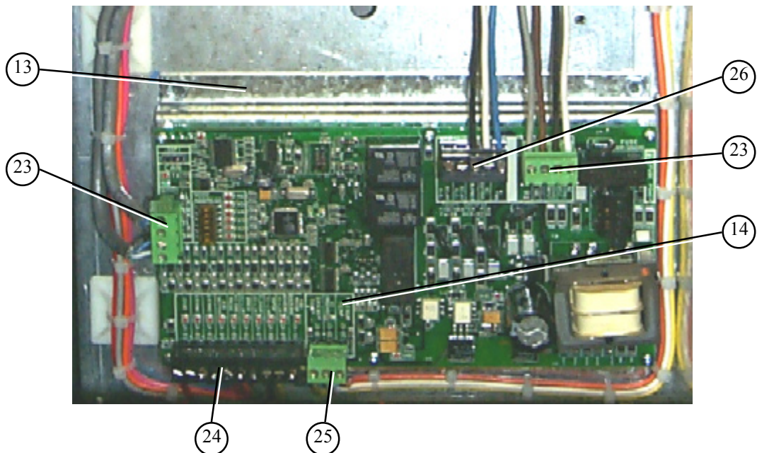
A detailed view of the heater board.
