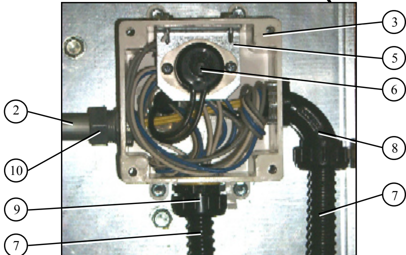
Lower plenum high limit junction box.
