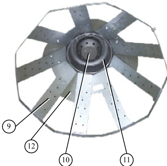
28" Fan heater burner assembly.
