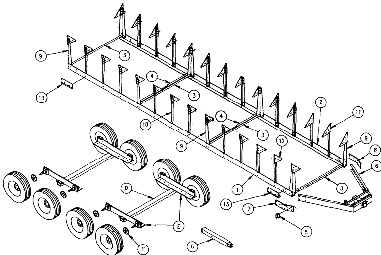
(14) TRANSPORT ASSEMBLY
