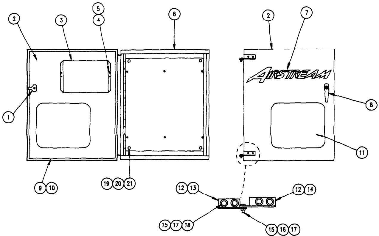
HINGE DETAIL
