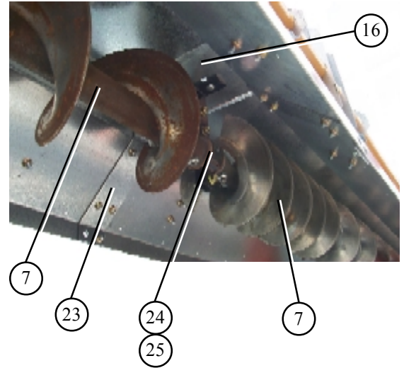
Top Auger bearing support (inside view).
