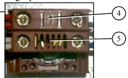
Detailed view of a single position switch.
