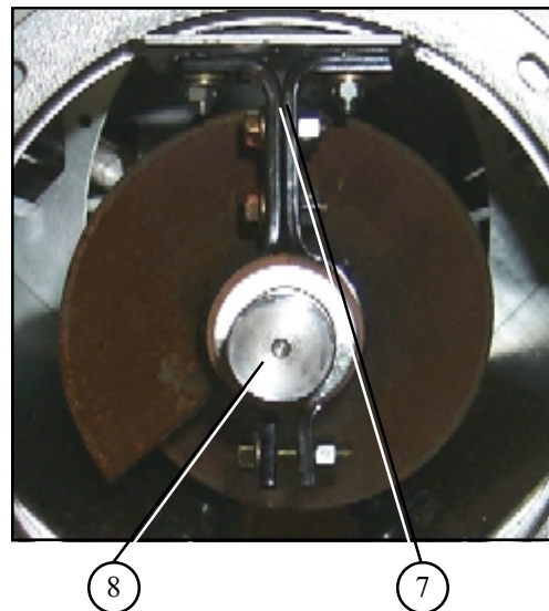
Bottom Auger rear bearing.
