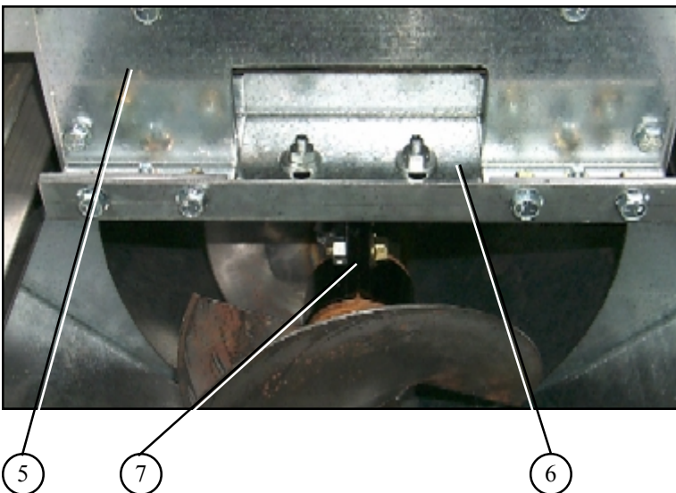
Bottom Auger center bearing and support.
