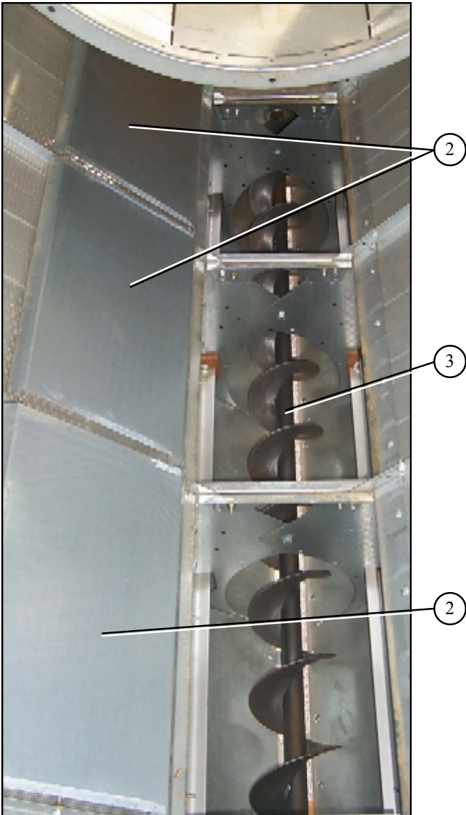
Bottom Auger center bearing and support.
