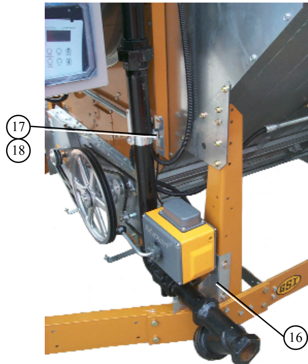
Supply line mounting brackets.
