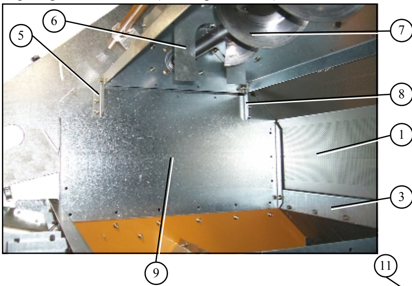
Top Auger with wet bin (switch paddle end).
