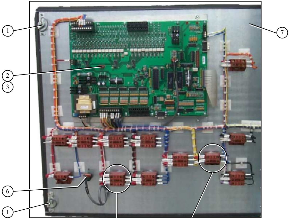
Network control panel (rear).
