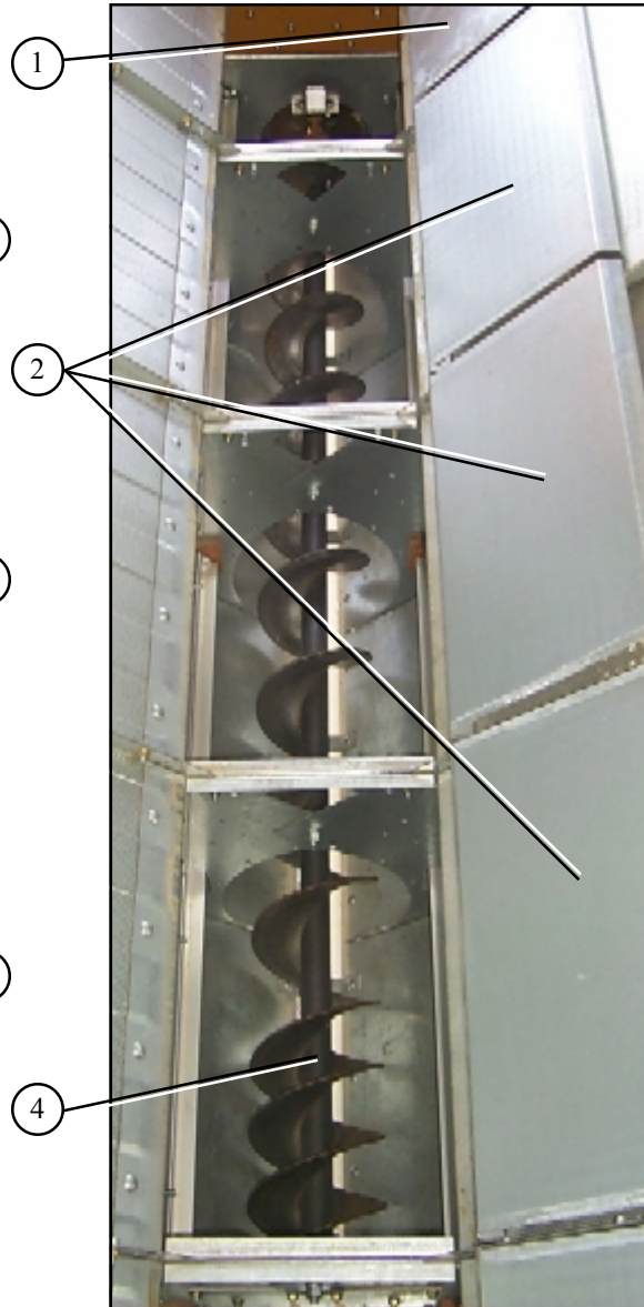
Bottom Auger rear bearing.
