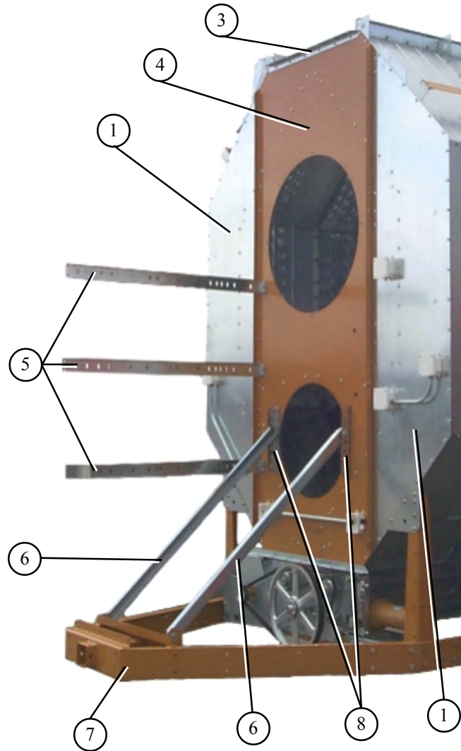
Front end panels & support arms.
