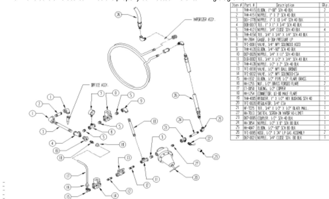
Exploded view of LP pipe train.
