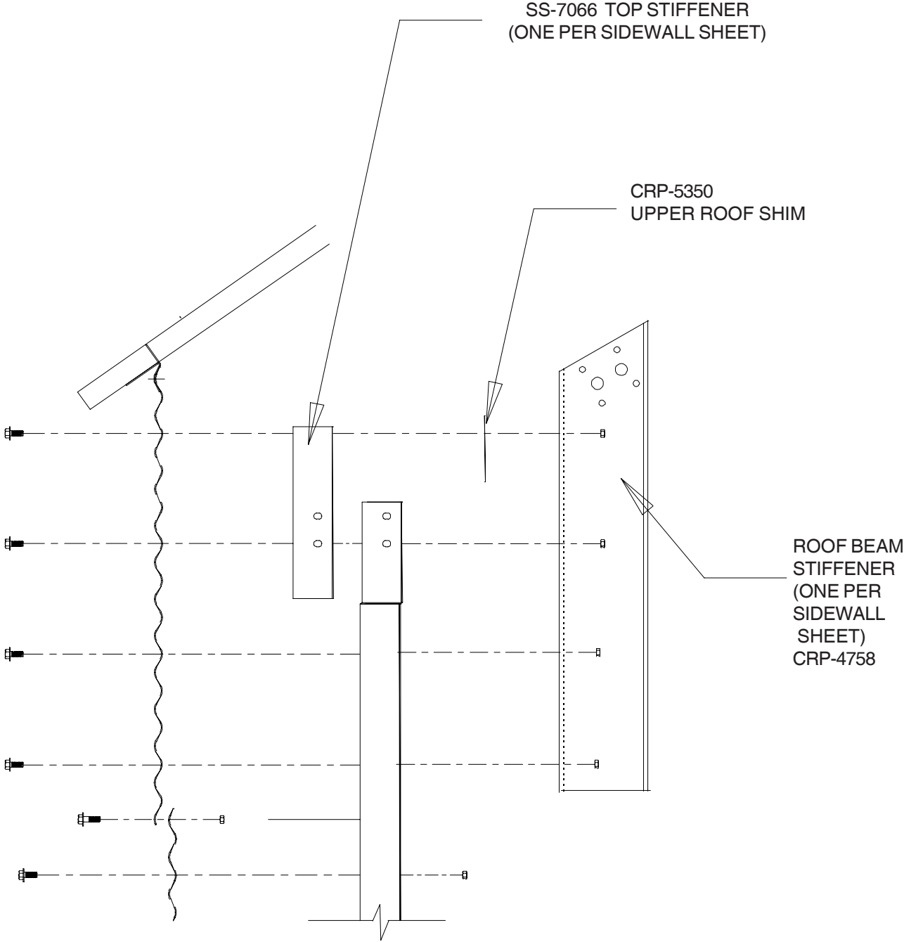
DETAIL A
