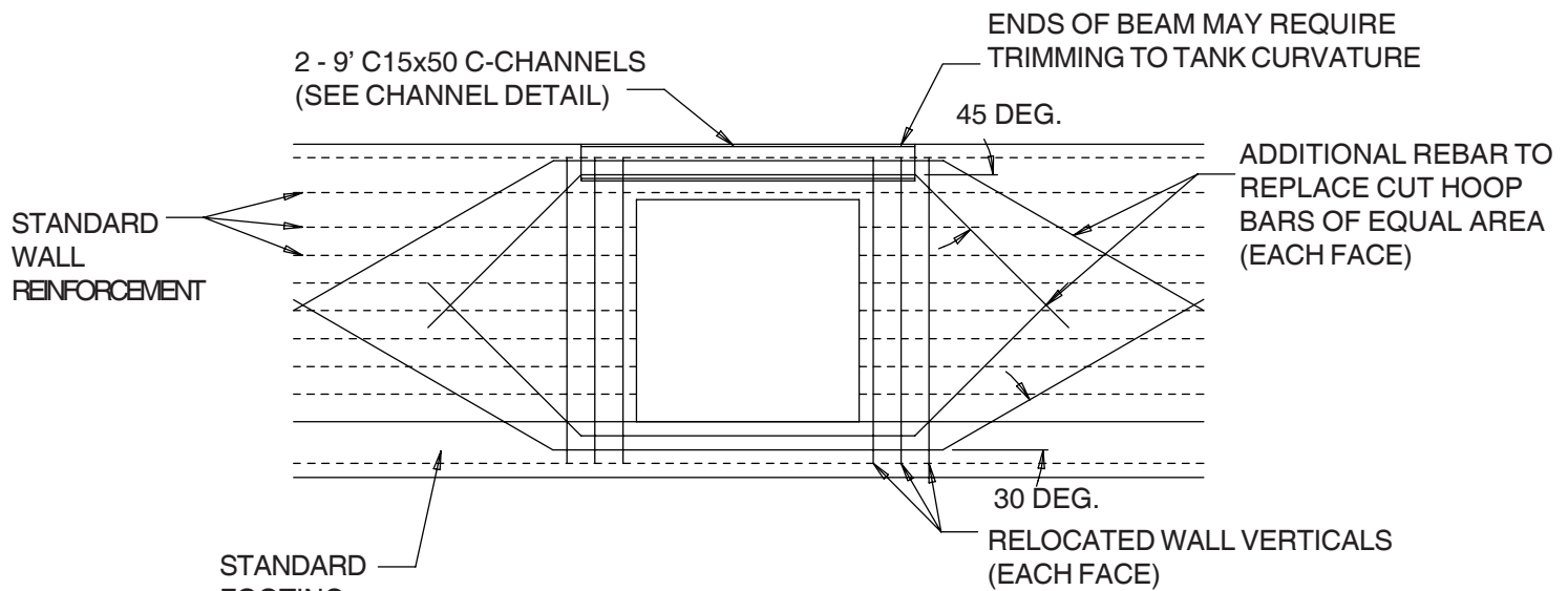
FRONT VIEW
