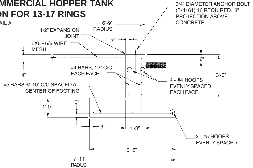
FOOTING DETAIL (NOTE: NOT TO SCALE)
