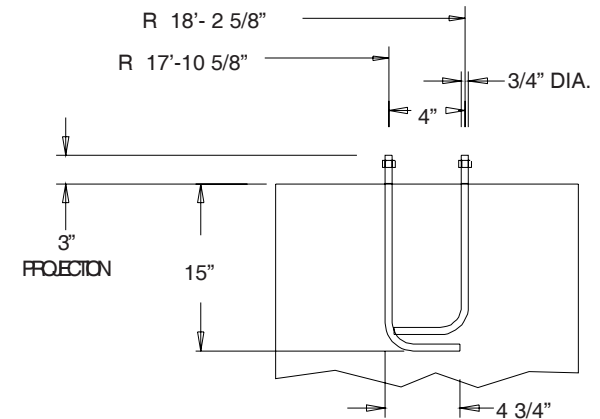
SECTION DETAIL
