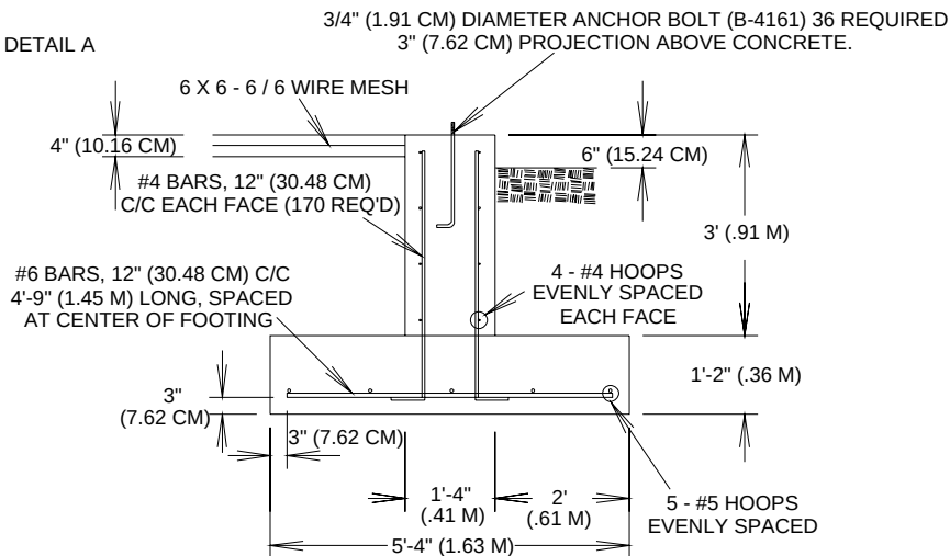
FOOTING DETAIL (NOTE: NOT TO SCALE)
