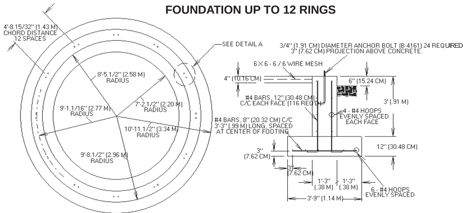
FOOTING DETAIL (NOTE: NOT TO SCALE)
