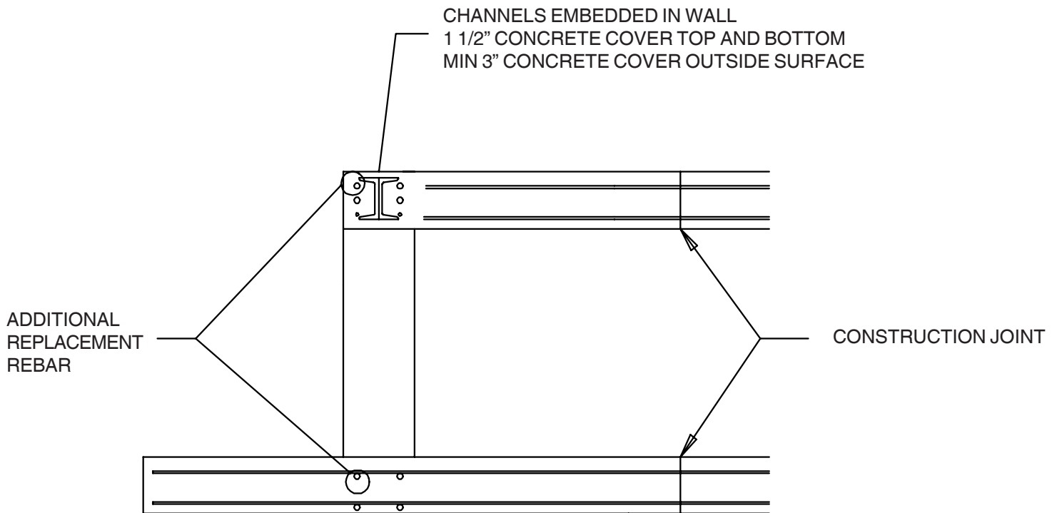
SIDE VIEW
