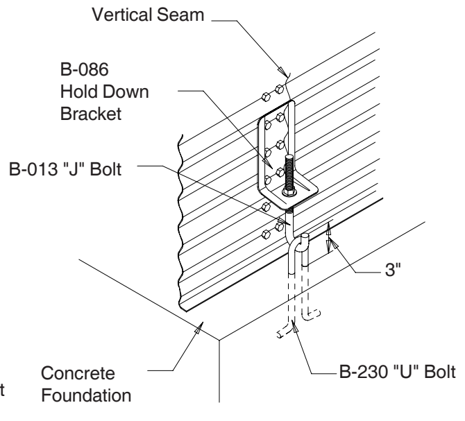
\"U\" BOLT/\"J\" BOLT Combination
