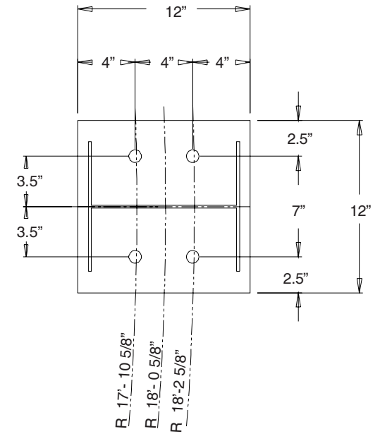
PLAN DETAIL
