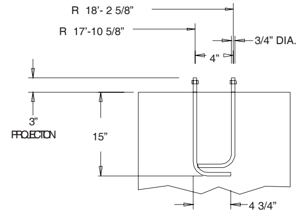
SECTION DETAIL
