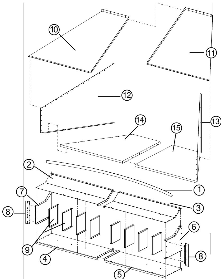
Figure 1: Transition for double inlet centrifugal fans
