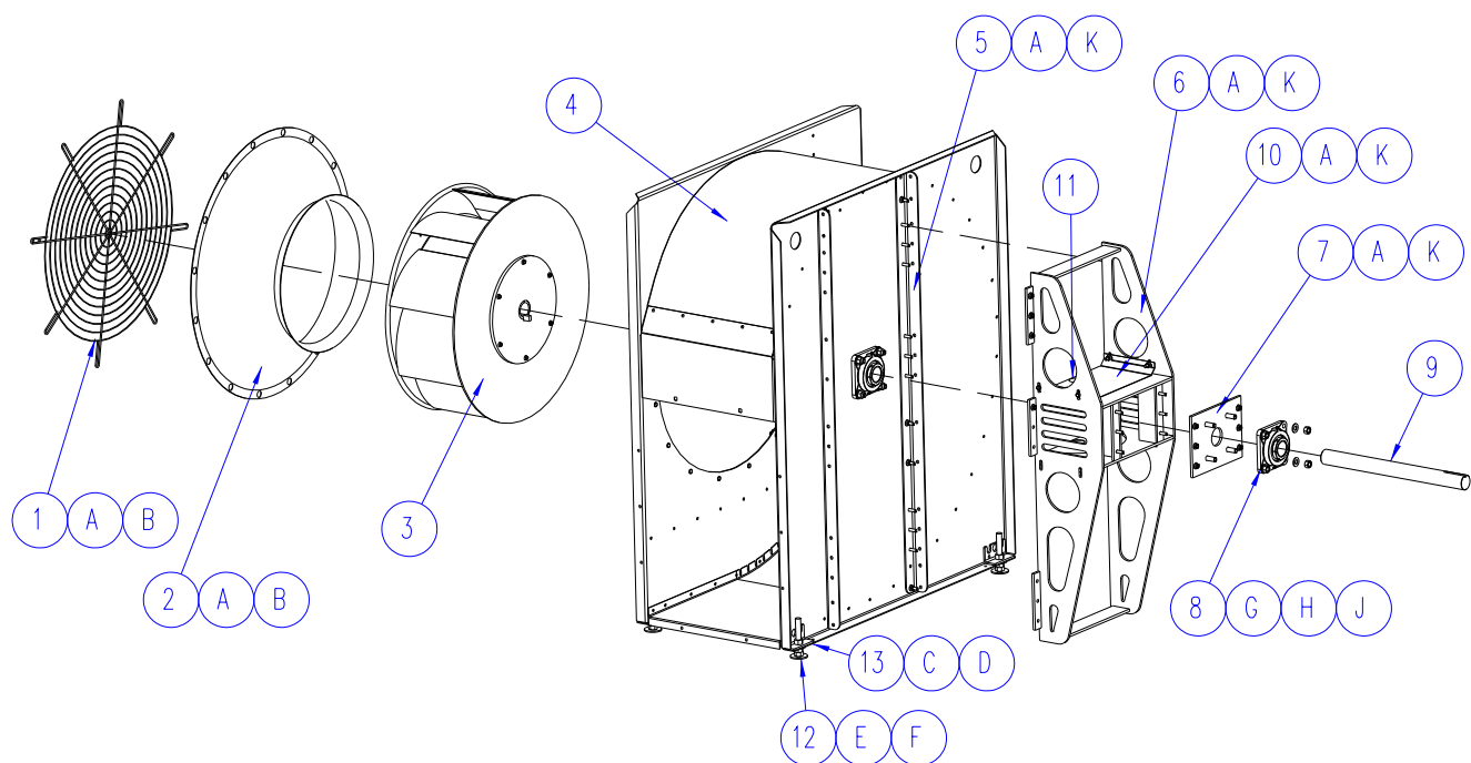
Single Inlet Direct Drive Fan - Main Assembly
