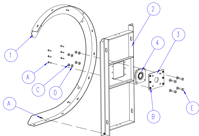
Internal Bearing Mount Assembly
