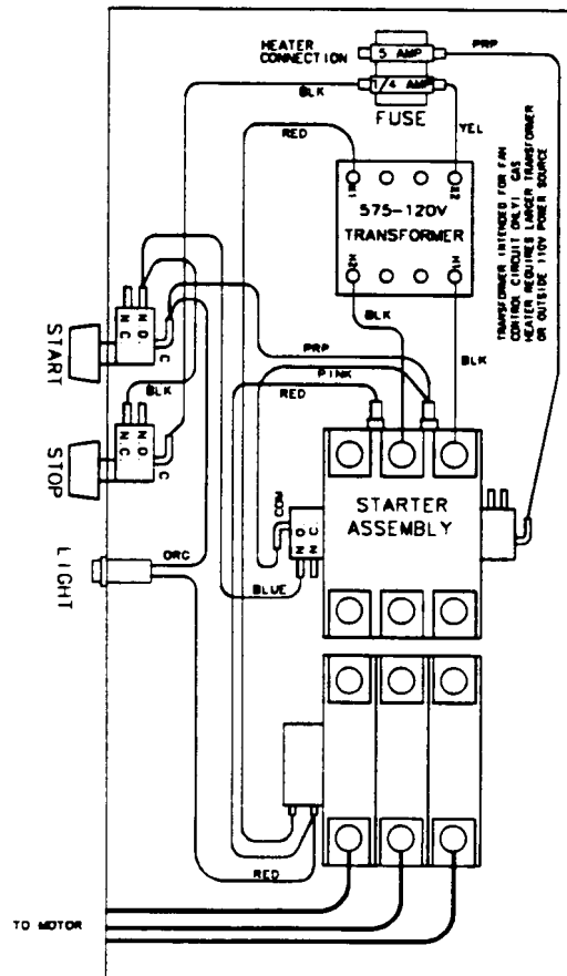
Wiring Diagram
