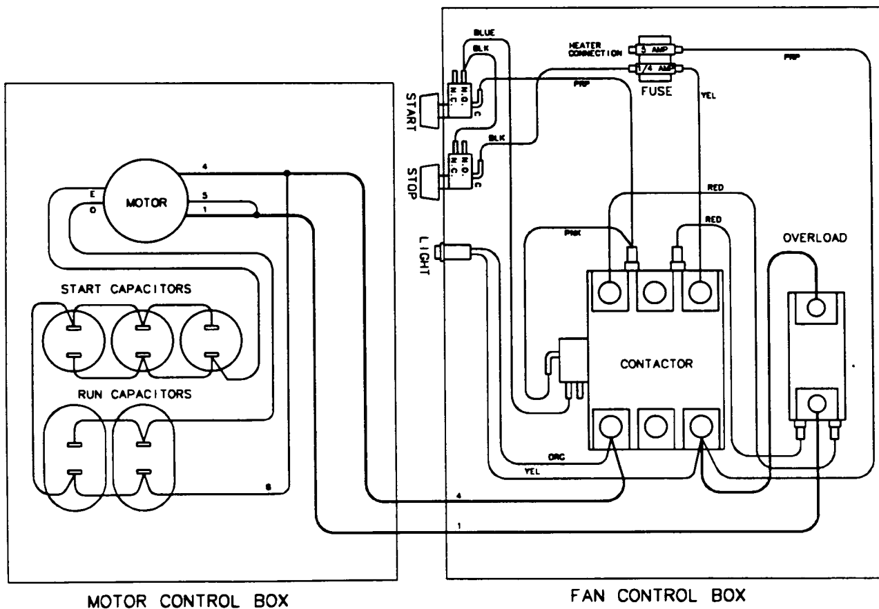
Wiring Diagram
