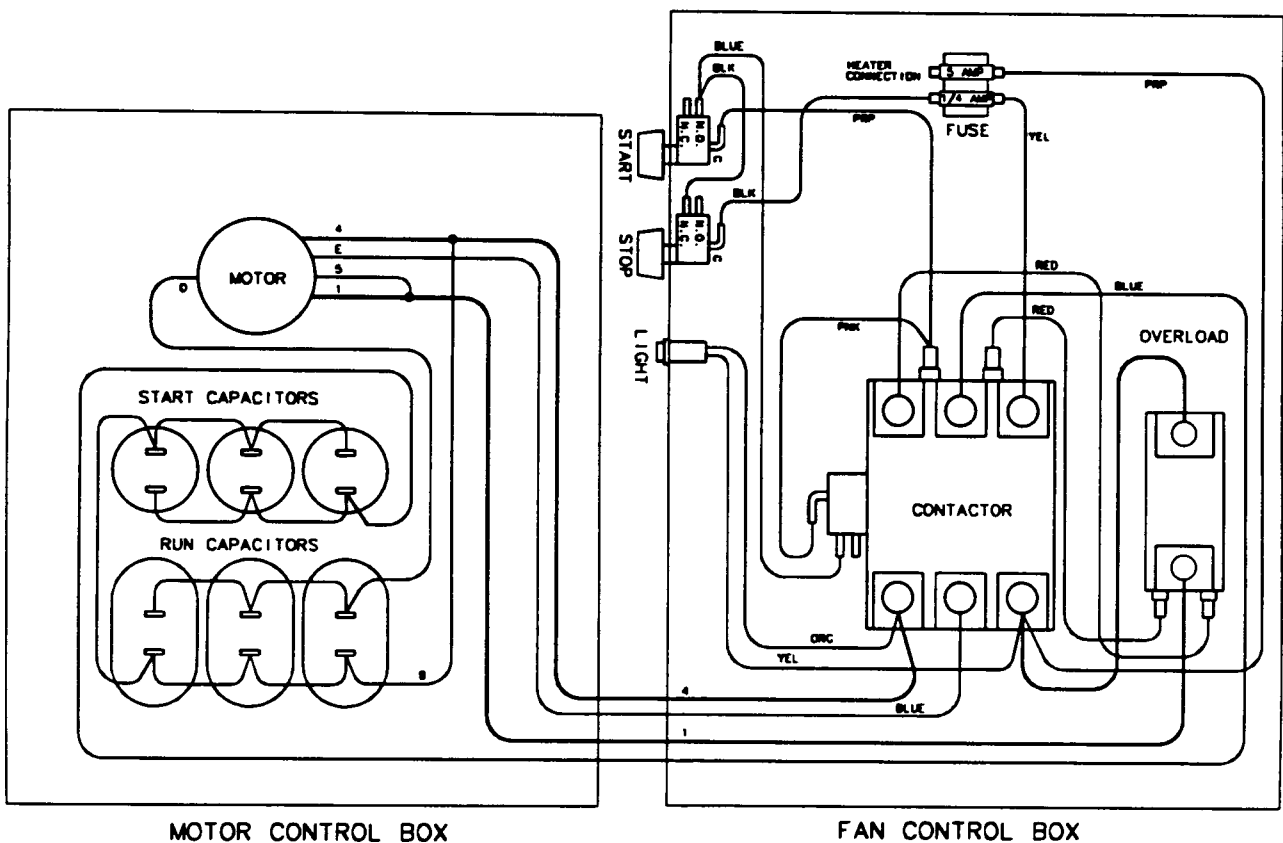
Wiring Diagram
