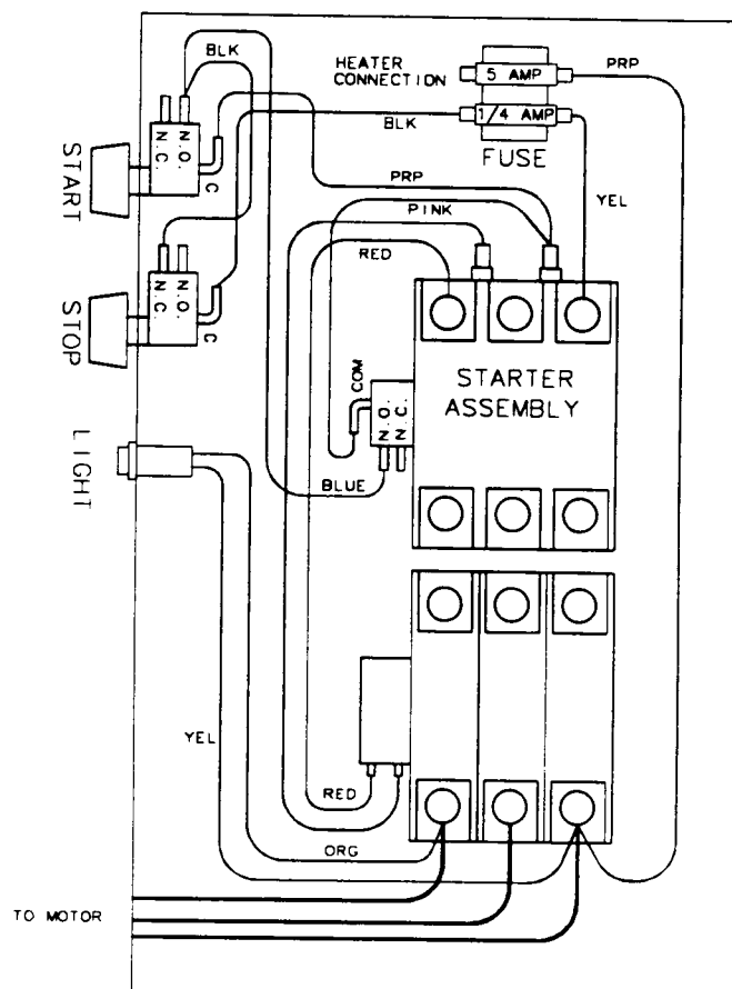
Wiring Diagram
